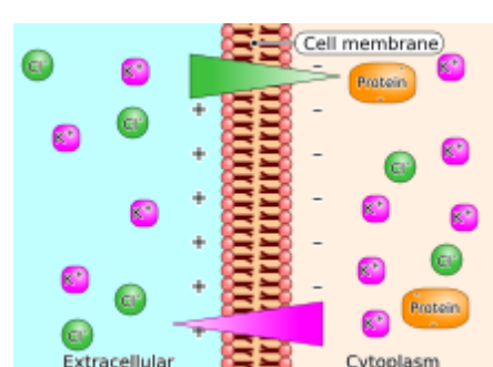
Schematic: Donnan equilibrium across a cell membrane
