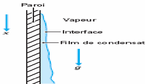
Figure VI.4. Condensation en film
