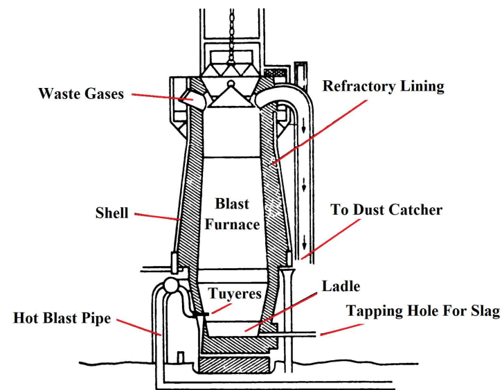
Cross-section of blast furnace
